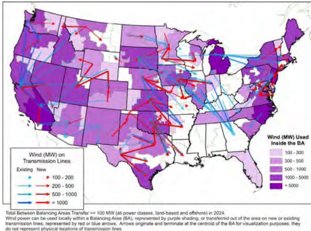
Figure A-16. Transport of wind energy over existing and new transmission lines projected for 2024
