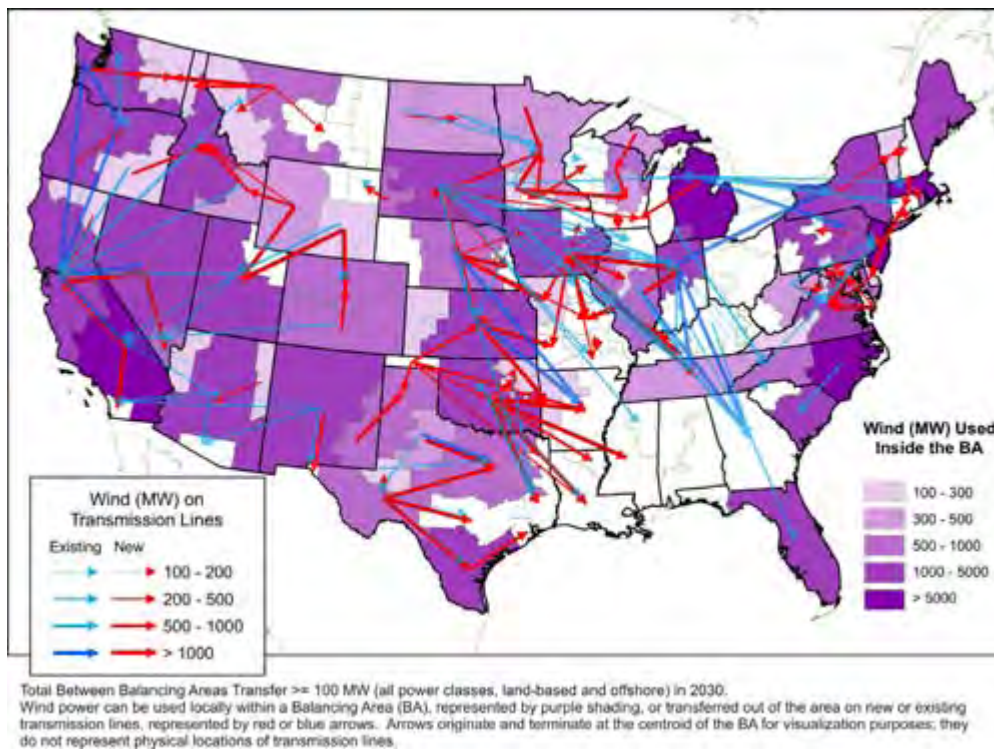
Figure A-17. Transport of wind energy over existing and new transmission lines projected for 2030
