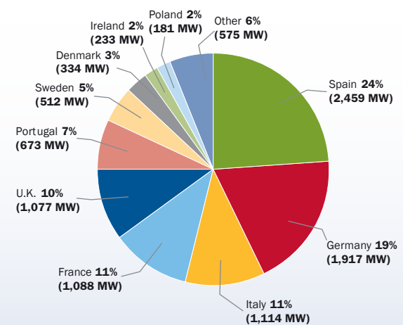
EU MEMBER STATE MARKET SHARES FOR NEW CAPACITY (AS OF END 2009). TOTAL 10,163 MW
