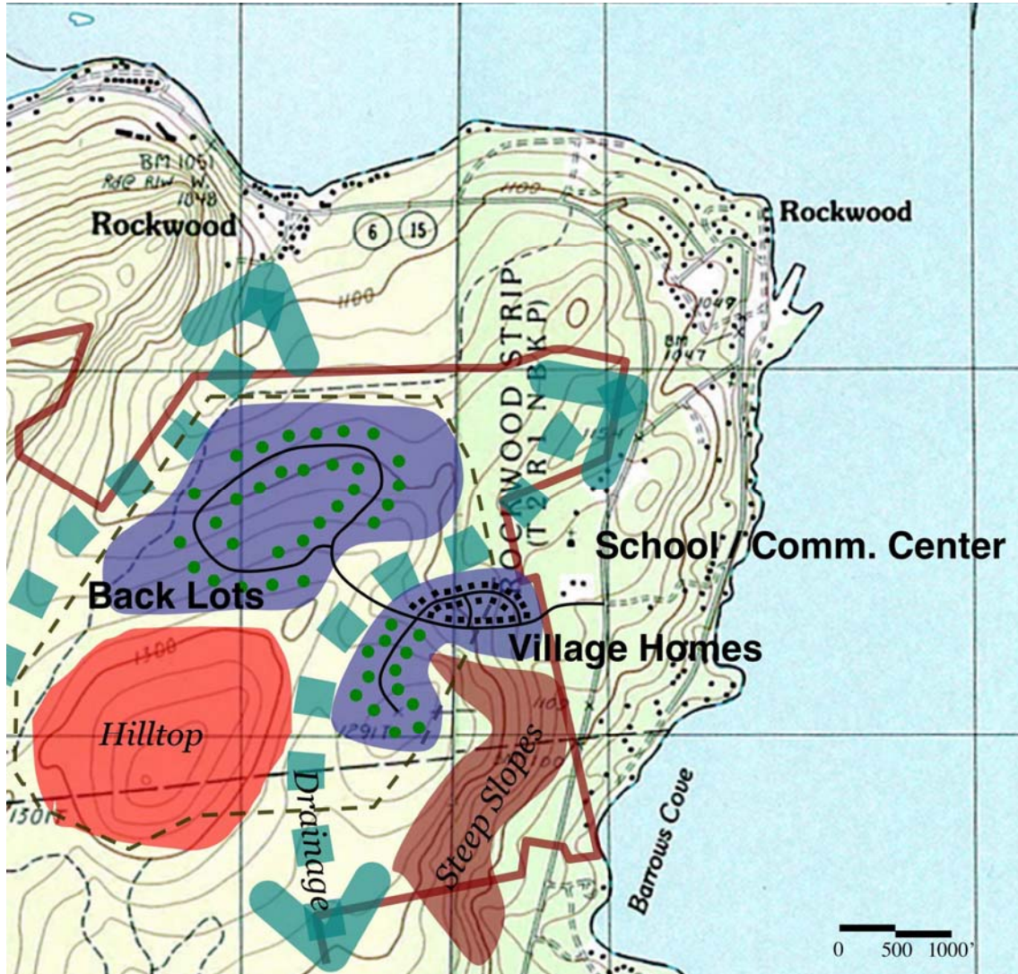
Sample conceptual layout for Rockwood development. Hilltop, steep slopes and streams protected. Village lots within walking distance of school and town center.
